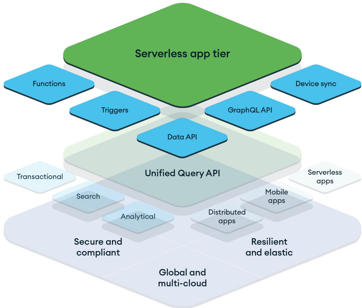
Figure 11.5: Unified key features of Atlas Application Services
