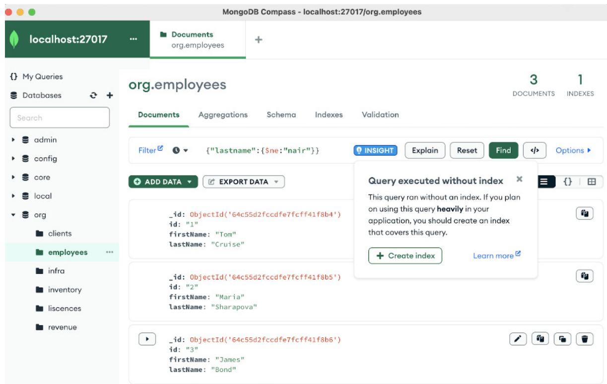
Figure 3.3: The optimization popup
