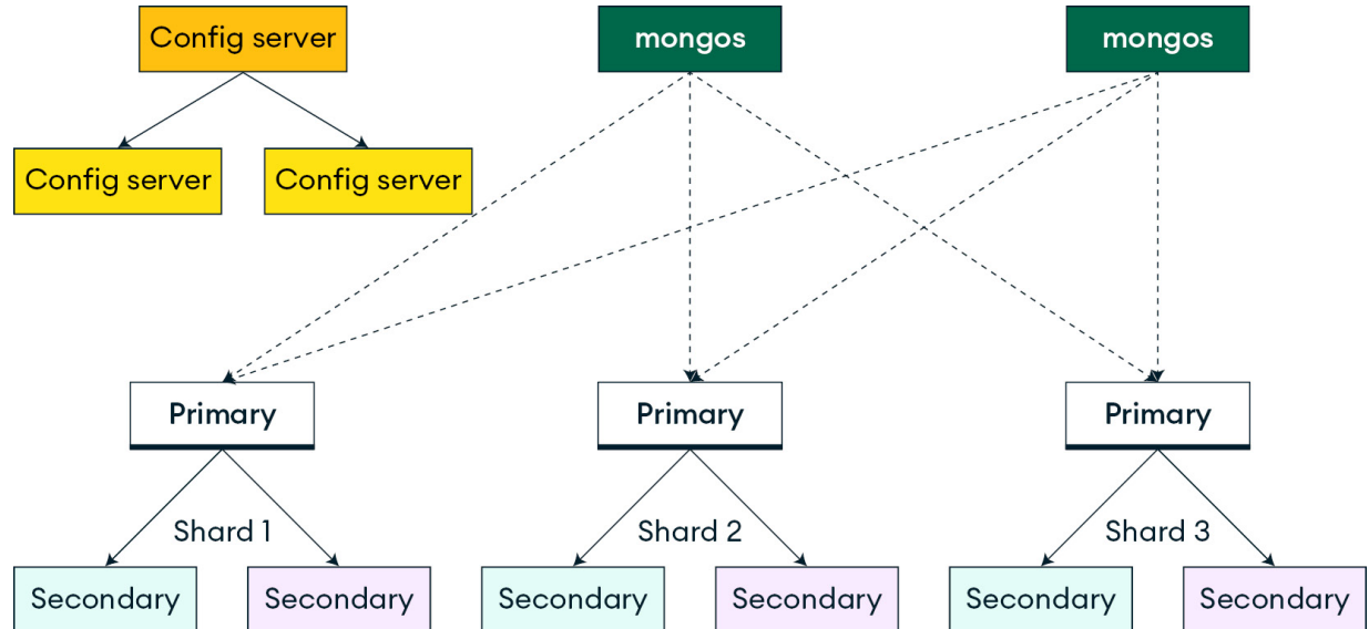
Figure 2.3: A sharded cluster
