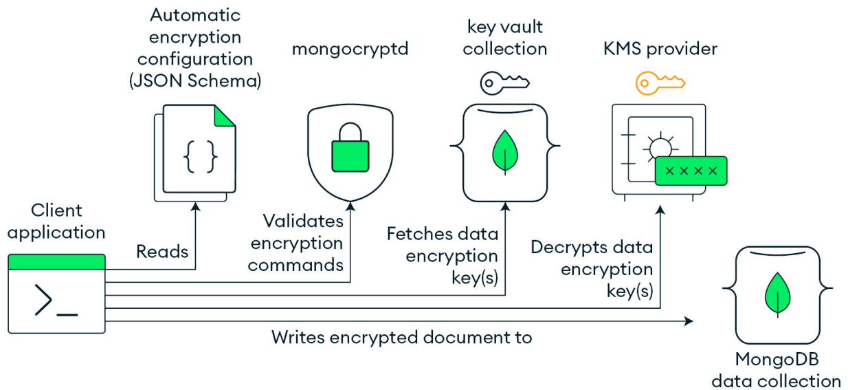
Figure 17.1: Steps to perform a write of field-level encrypted data
