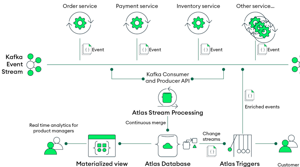
Figure 11.6: Atlas Stream Processing interfacing with various data sources
