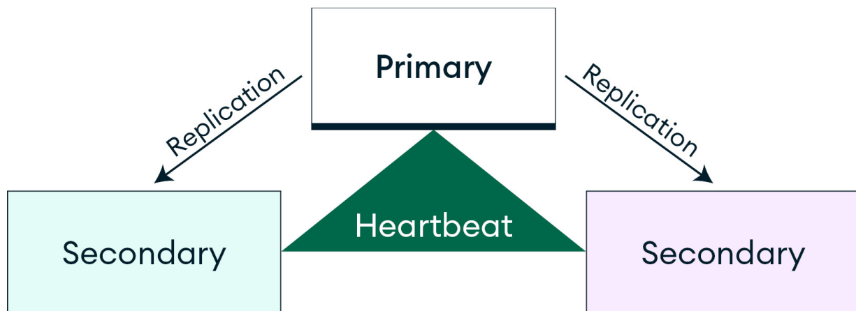
Figure 2.1: A replica set
