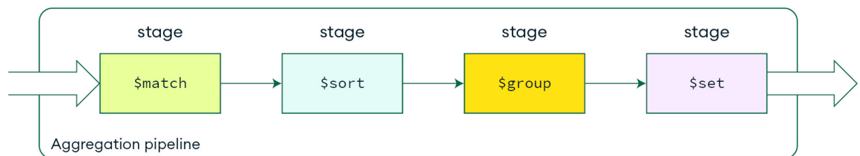
Figure 8.1: The aggregation pipeline structure, including stages
