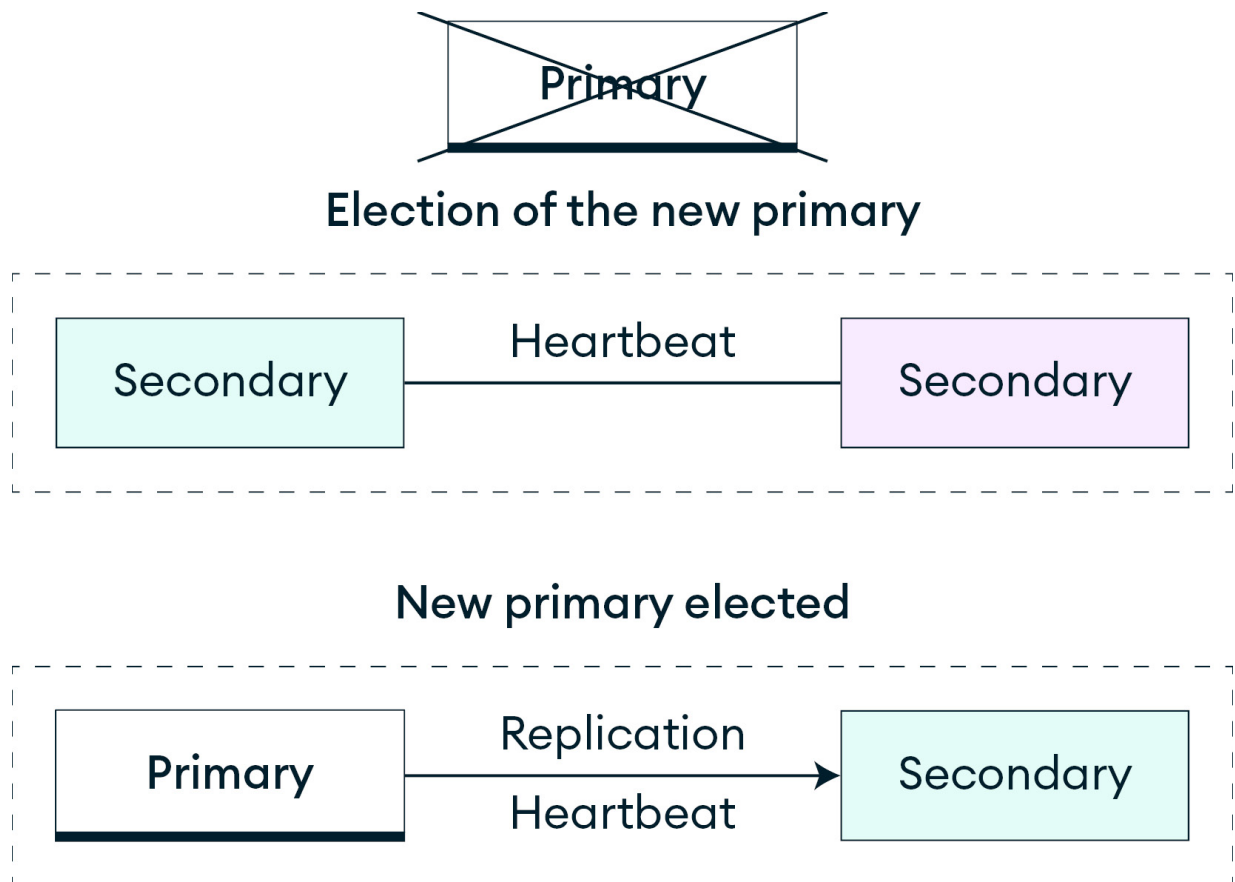
Figure 2.2: Electing a new primary
