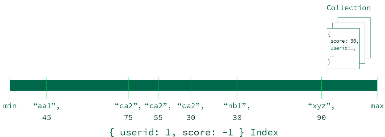
Figure 10.4: An example of a compound index
