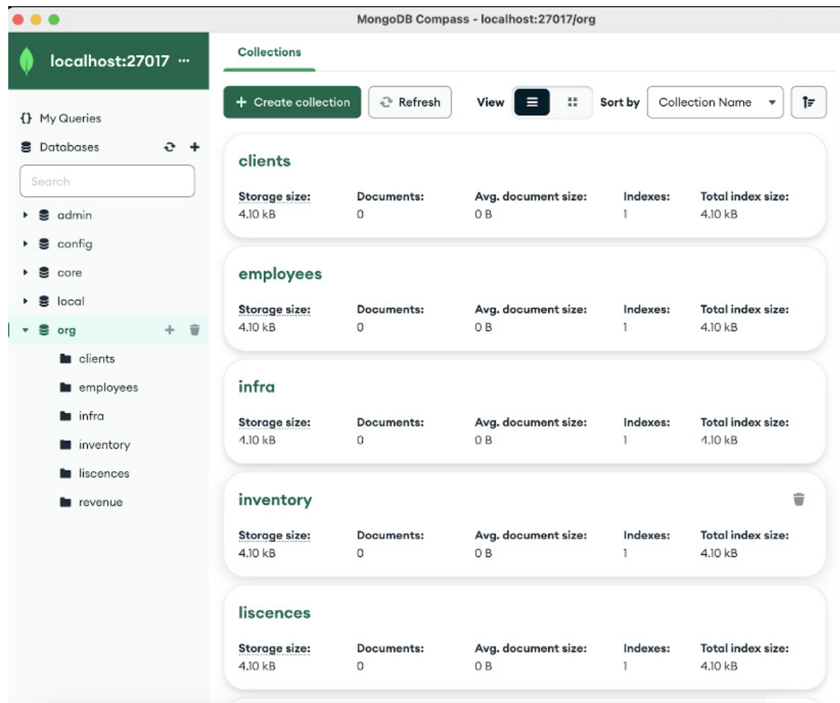
Figure 3.2: The MongoDB Compass environment
