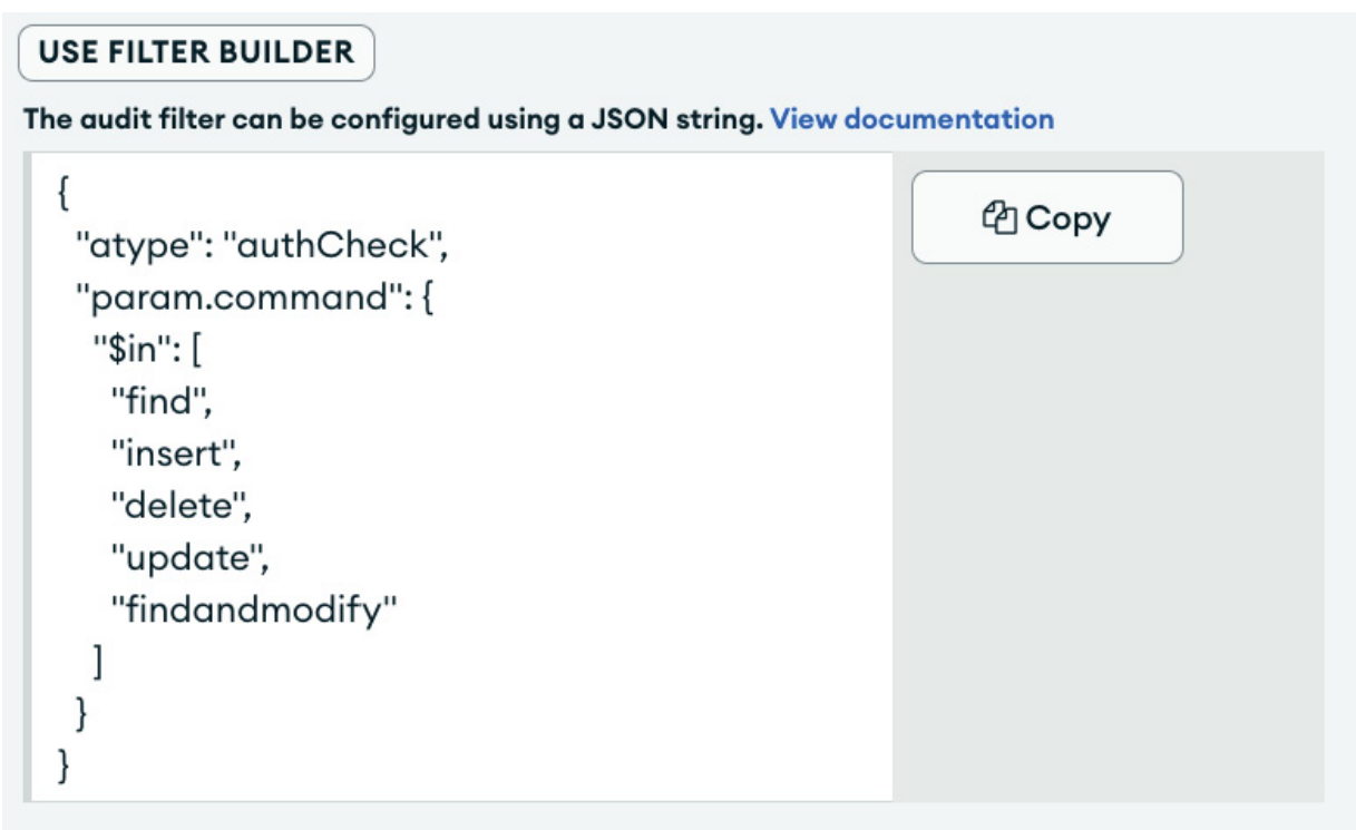
Figure 16.3: Applying audit filters
