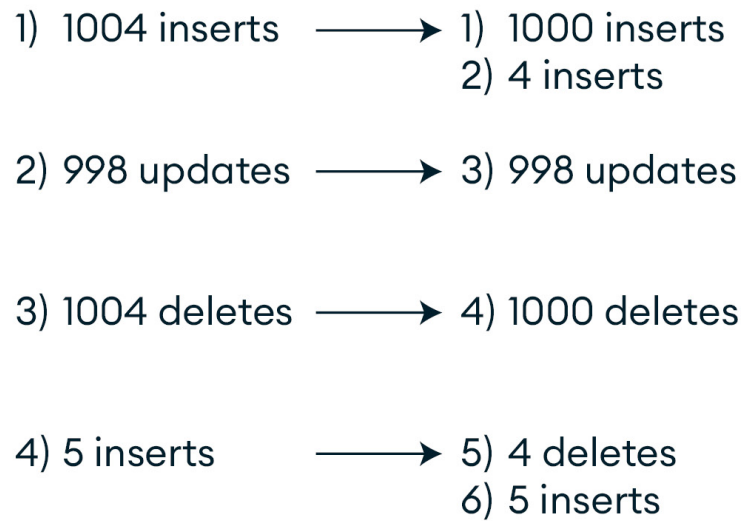
Figure 5.2: Bulk operations ordering
