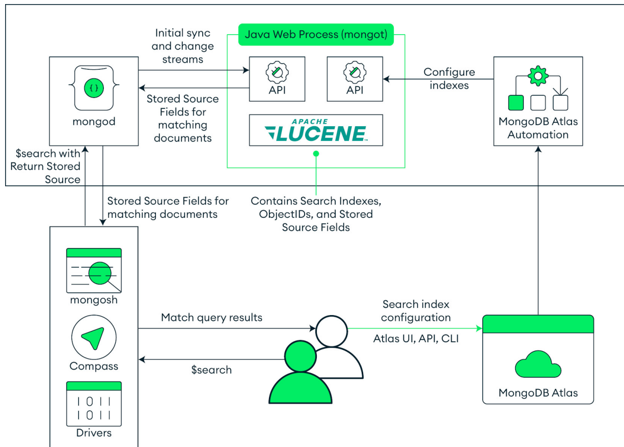
Figure 13.5: Optimized Atlas Search query processing
