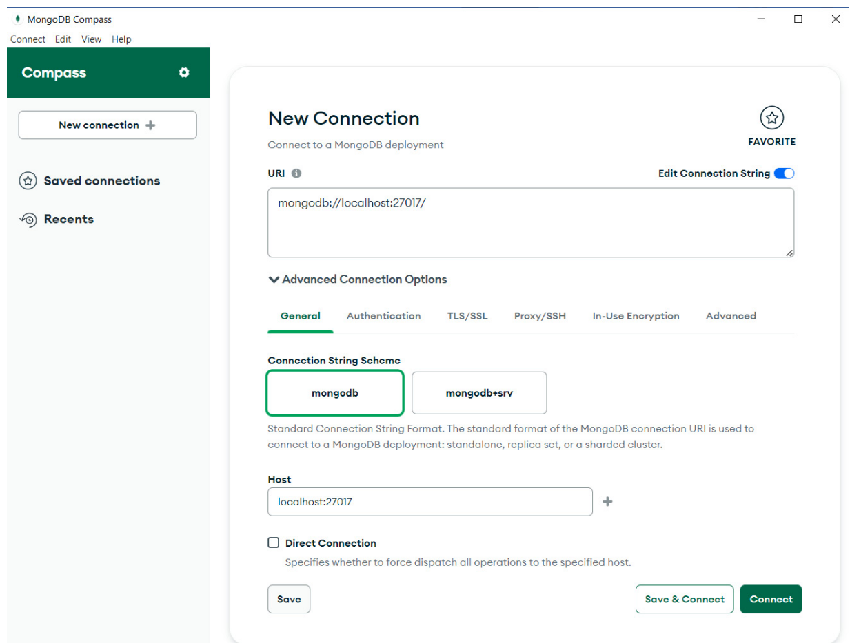
Figure 3.1: New connection configuration
