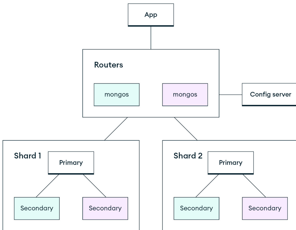
Figure 1.1: Replicated partitions set with primary and secondary nodes
