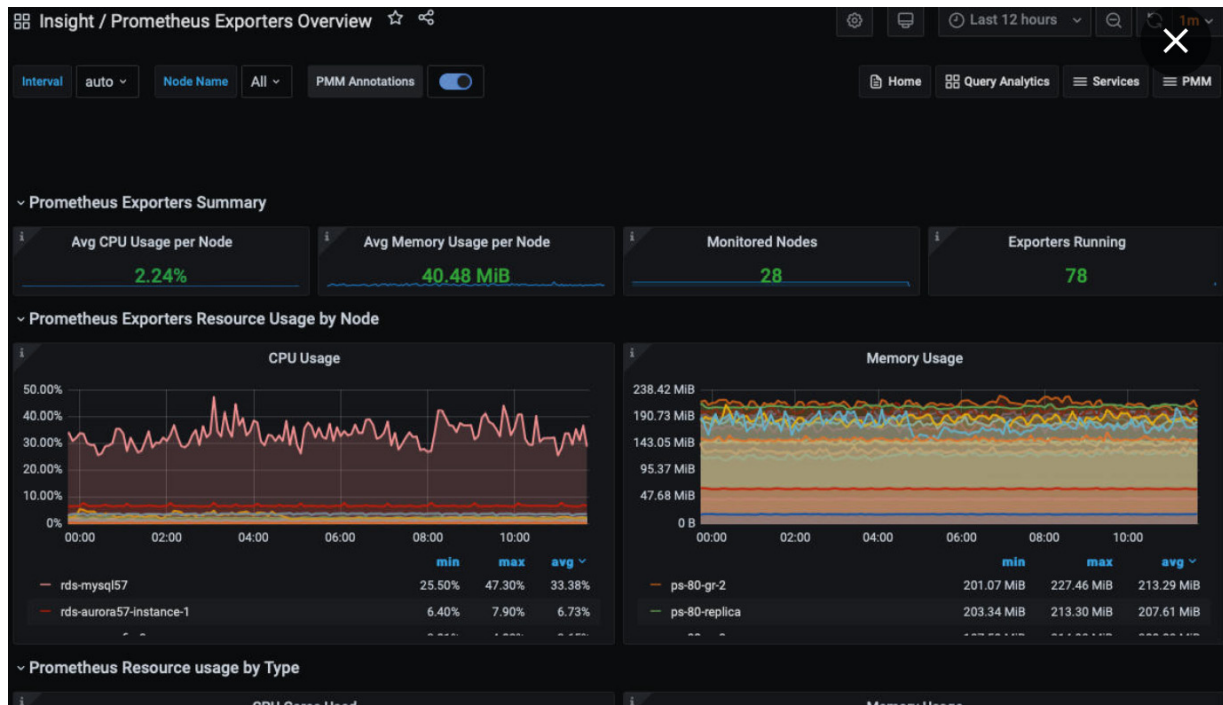
Figure 14.7: Prometheus integration
