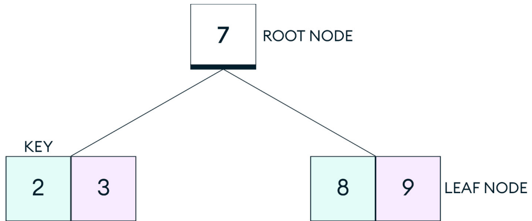
Figure 10.1: The B-tree data structure
