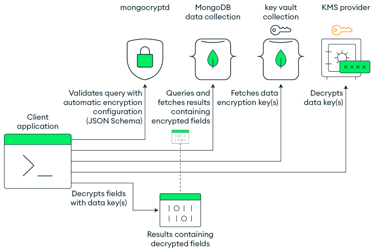
Figure 17.2: Steps taken to query and decrypt field-level encrypted data
