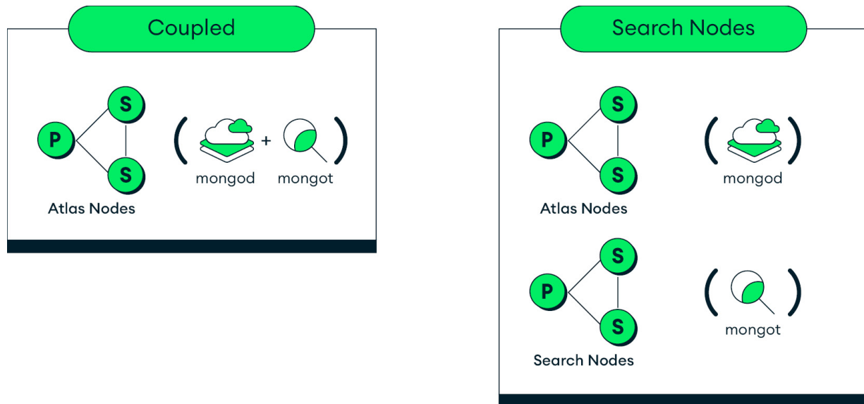
Figure 13.3: Atlas Search Node configurations
