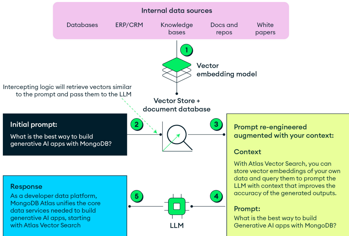
Figure 11.4: Atlas Vector Search in MongoDB
