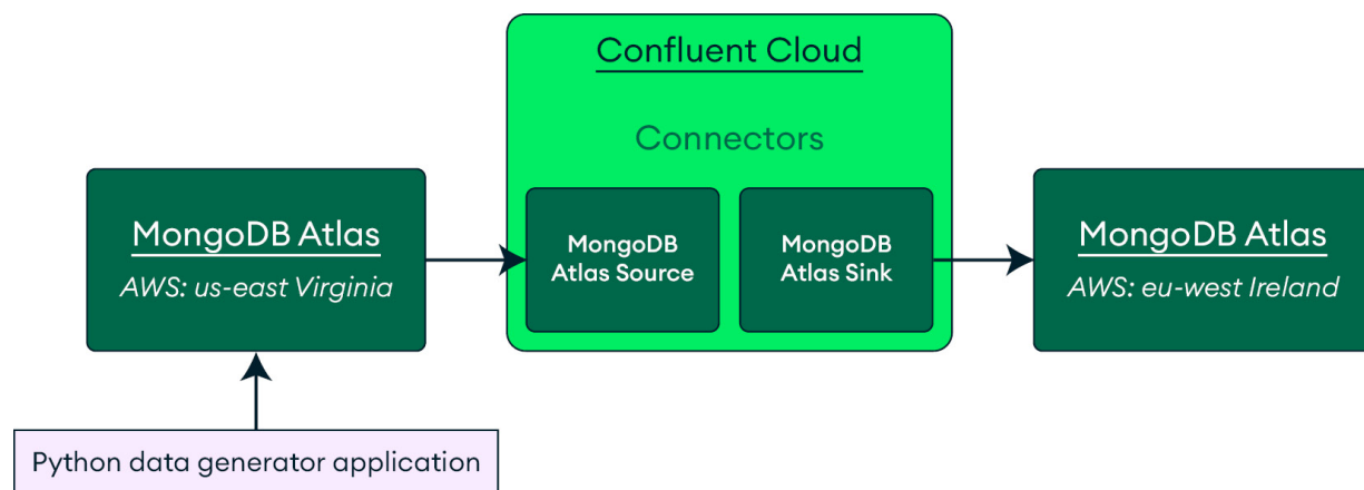
Figure 14.10: Confluent Kafka between Atlas clusters
