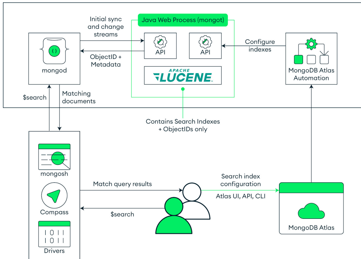
Figure 13.4: Atlas Search query processing
