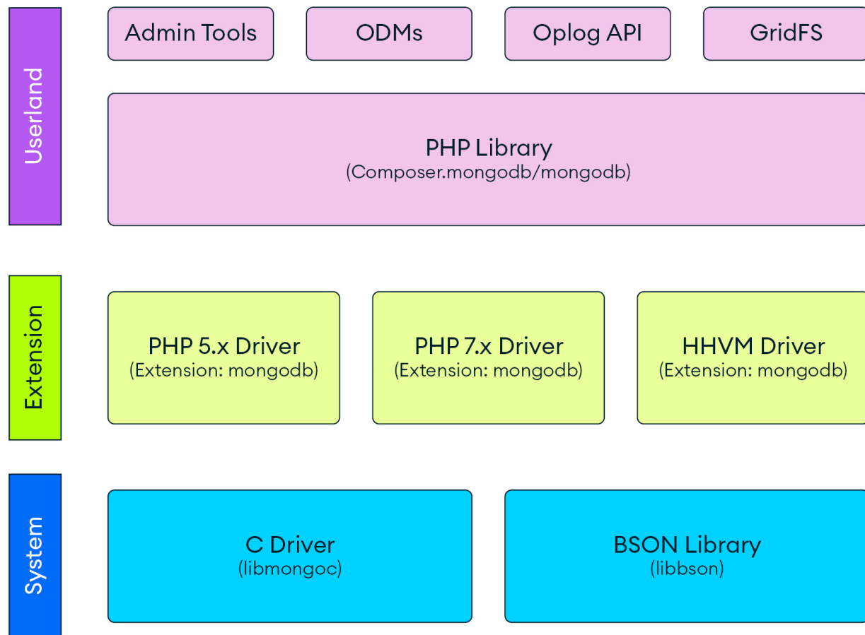
Figure 4.1: PHP driver architecture
