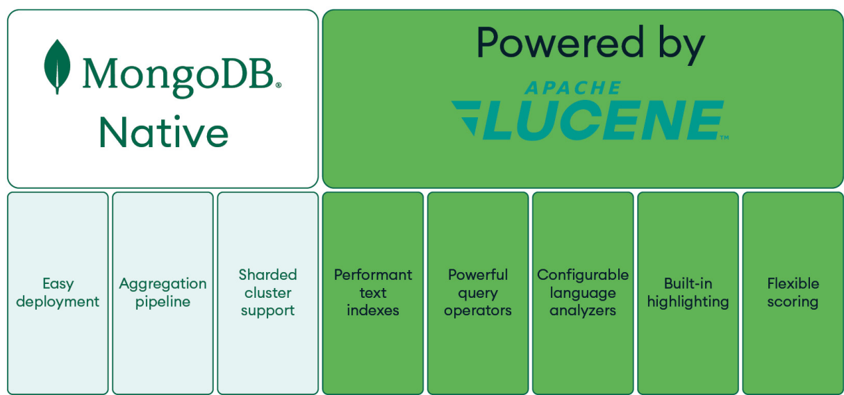
Figure 13.1: Atlas Search
