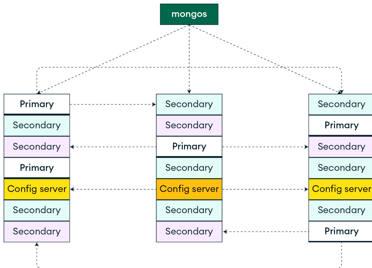
Figure 2.4: Microsharding configuration
