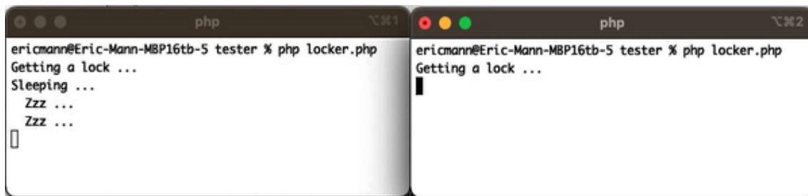
Figure 10-1. Two processes cannot acquire the same lock on a single file
