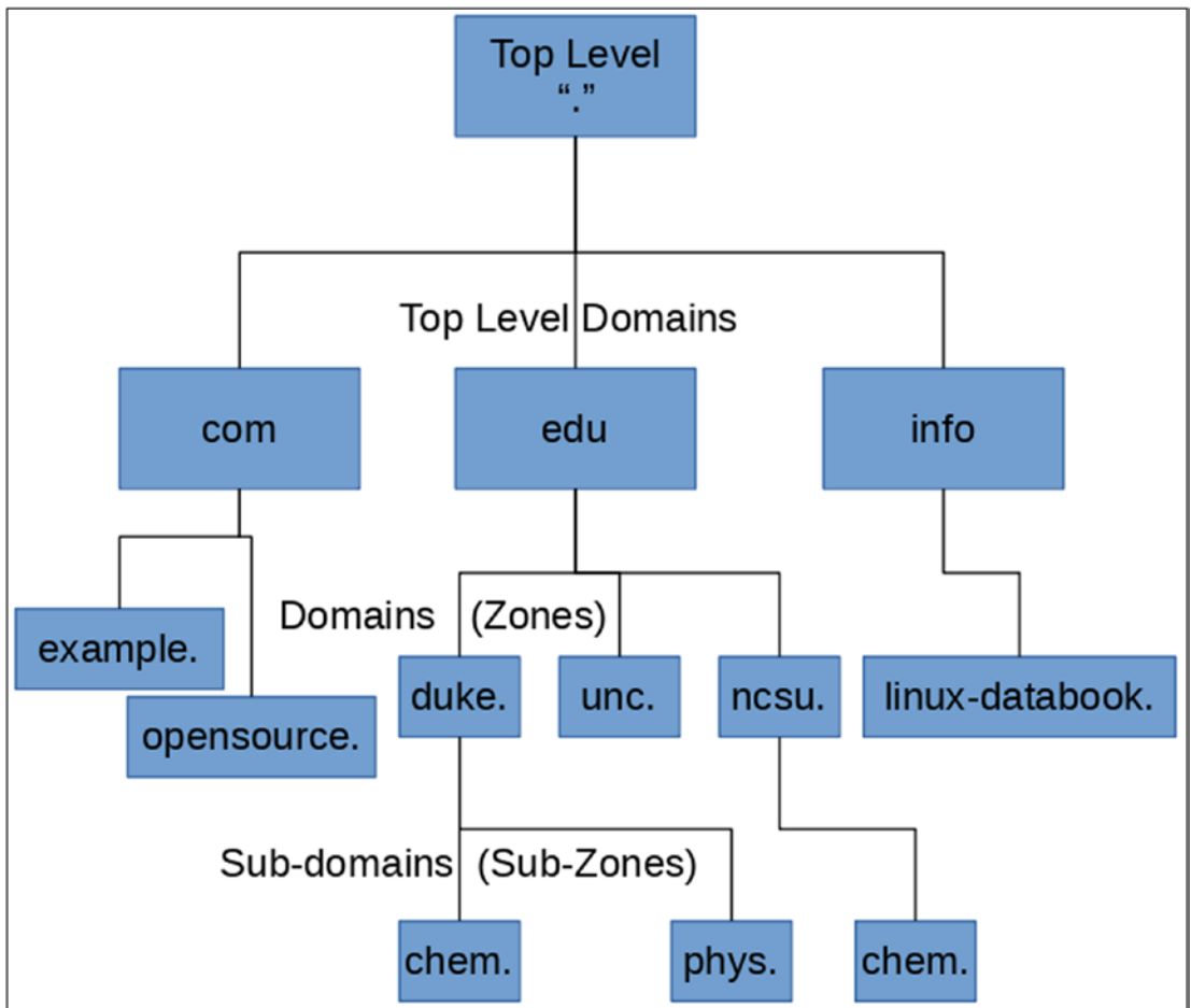
Figure 43-2. A very simplified representation of the DNS database hierarchical structure
