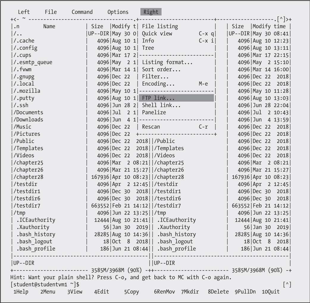
Figure 56-1. Select the FTP link to connect with the VSFTP server in standard FTP mode
