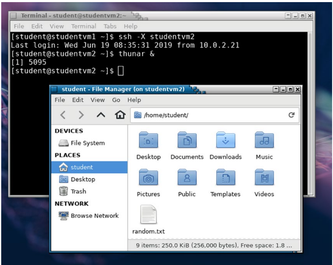
Figure 45-1. Using X-forwarding via SSH to display the Thunar file manager running on StudentVM2 in a window on the desktop of StudentVM1
