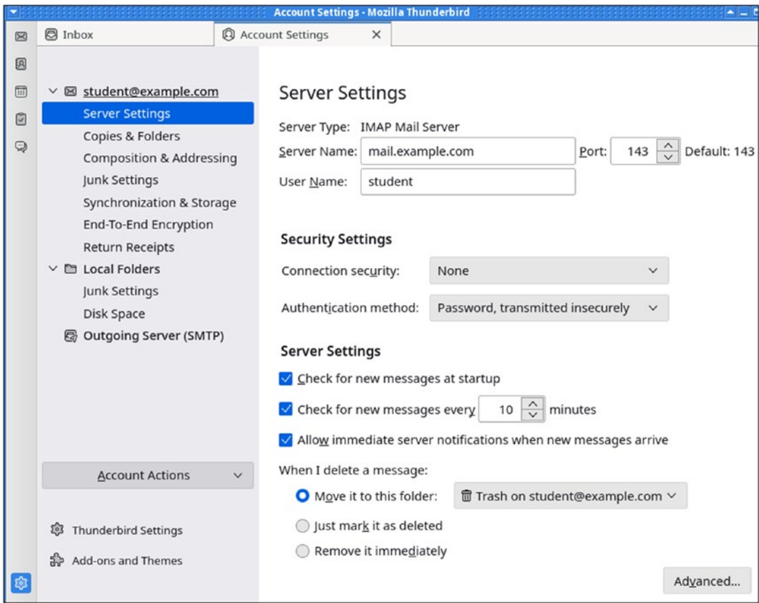
Figure 49-14. IMAP server settings for Thunderbird
