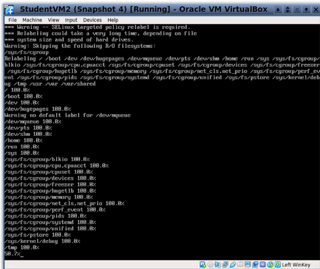
Figure 46-5. SELinux relabels system objects during a reboot
