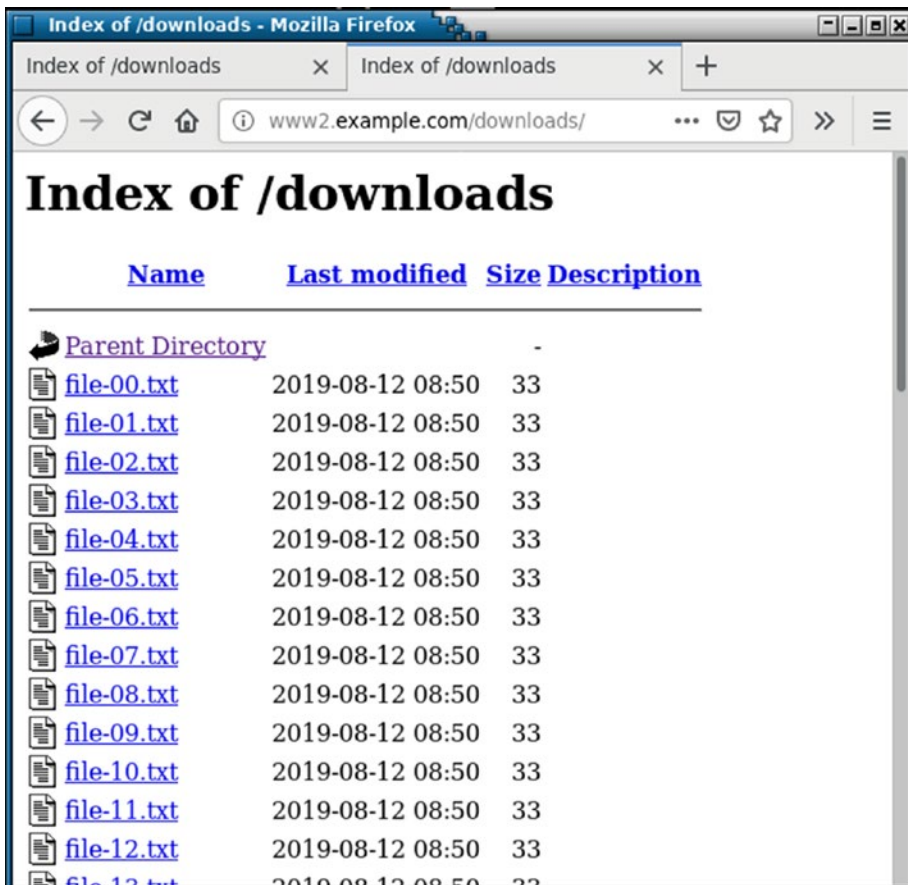
Figure 56-4. Using the Apache web server to share files displays a sortable index
