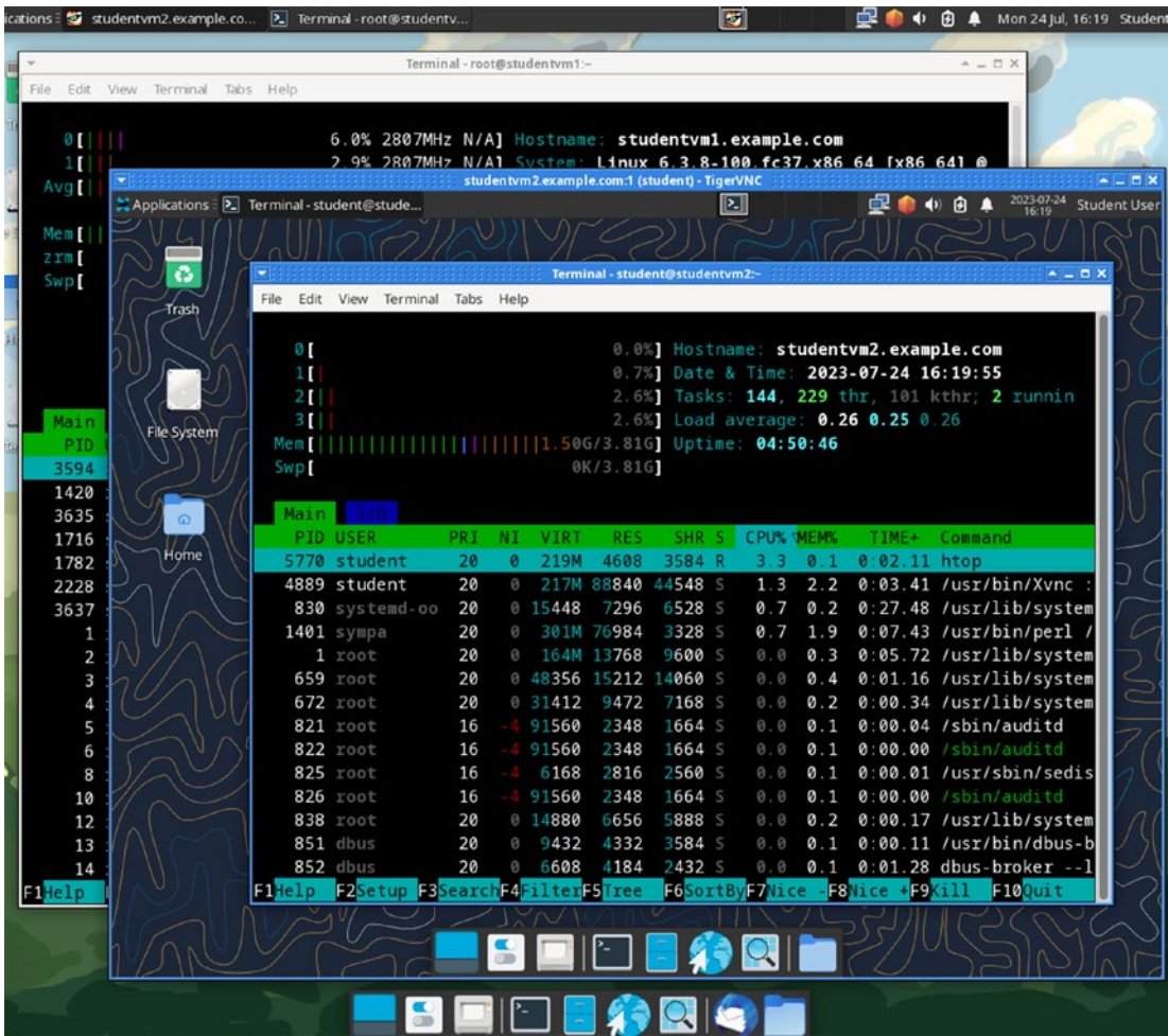
Figure 54-2. The StudentVM2 desktop via TigerVNC as seen on the StudentVM1 desktop
