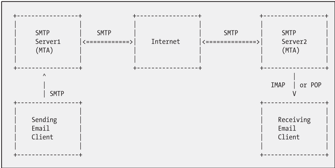
Figure 48-1. The flow of data for email messages
