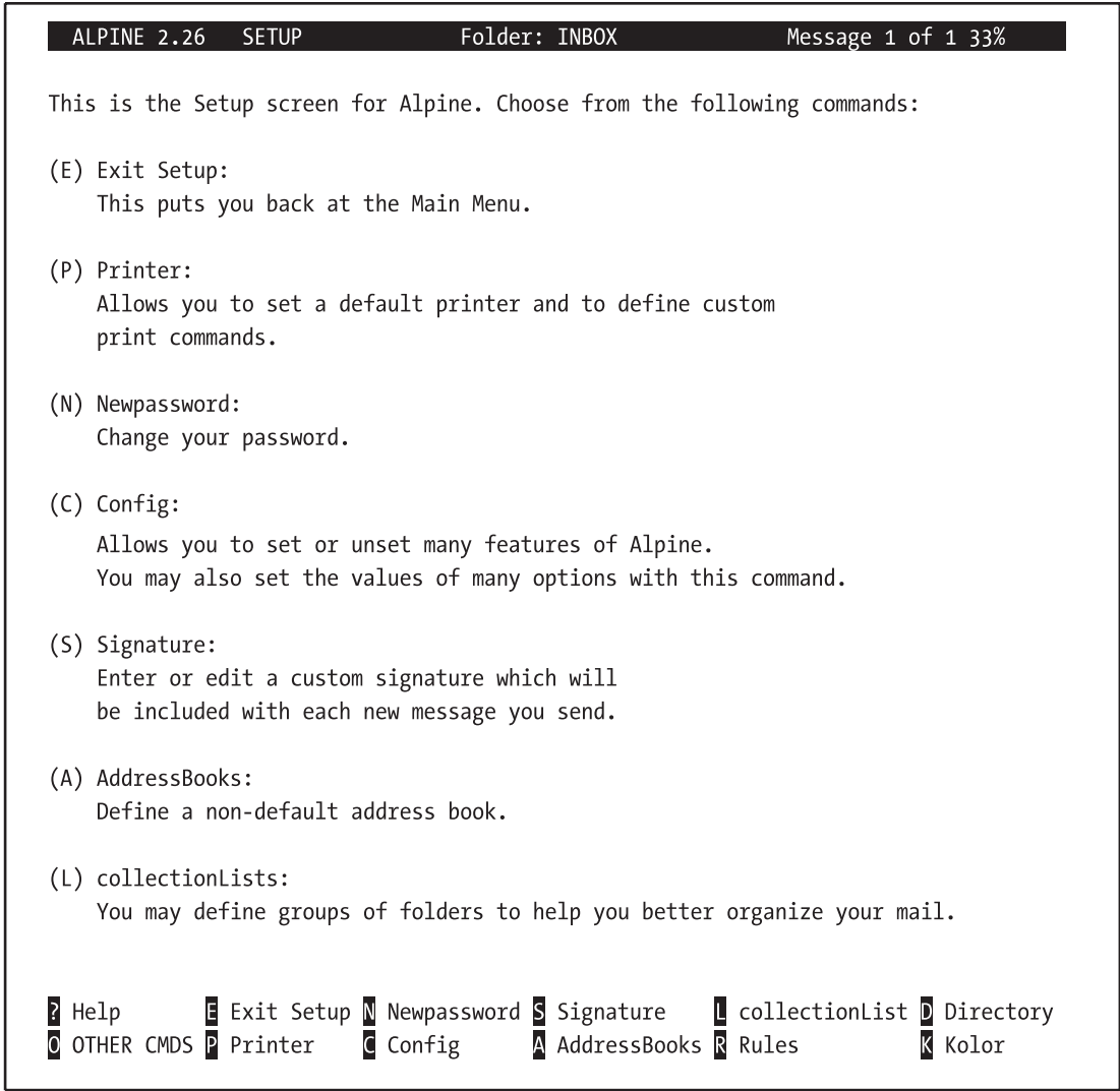
Figure 49-2. The Setup menu groups many setup options together so they can be easily found. Use Page Down and Page Up to scroll through the commands if you can't see them all
