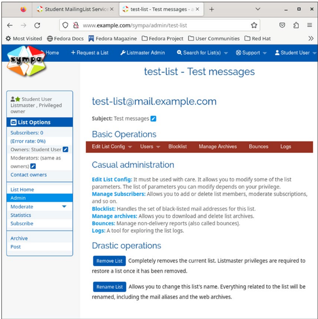
Figure 53-4. The list administration dialog for the new list
