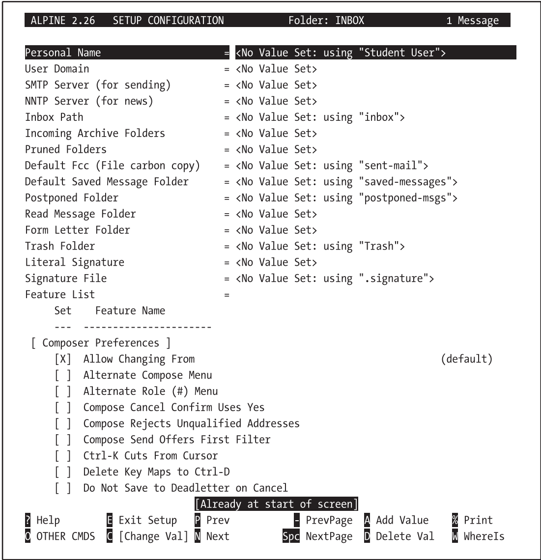
Figure 49-3. The first page of the Setup Configuration menu contains those few settings required to configure Alpine to send and receive email
