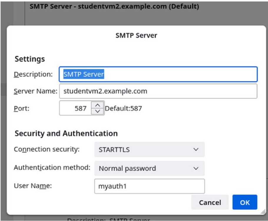
Figure 49-20. SMTP AUTH configuration for Thunderbird
