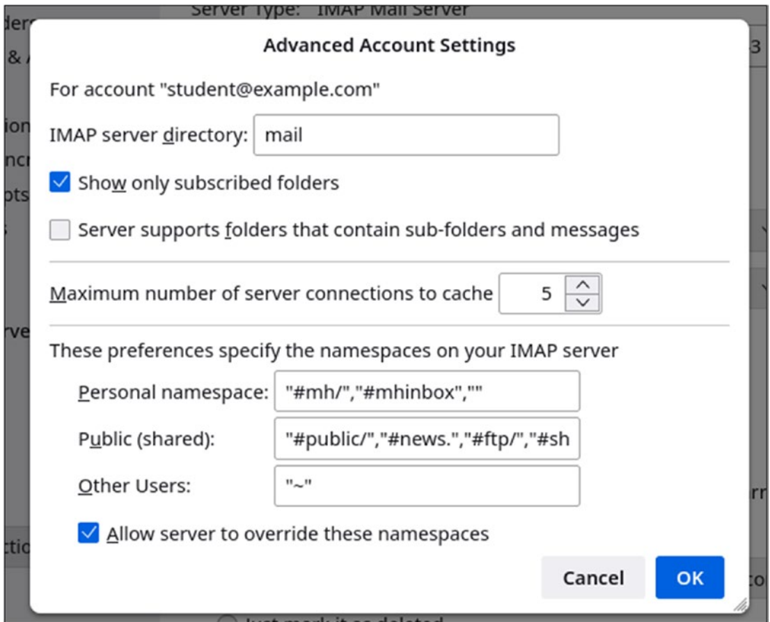
Figure 49-15. Be sure to enter “mail” in the IMAP server directory field
