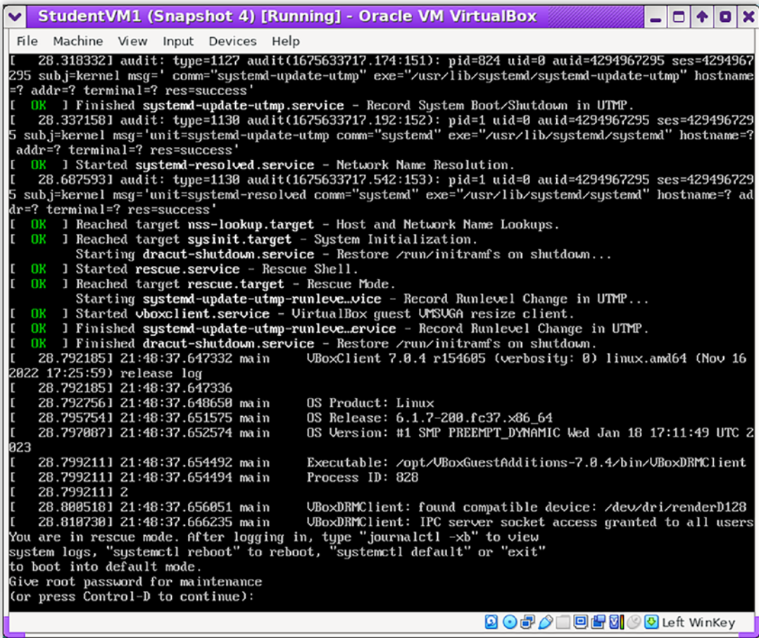
Figure 16-12. After booting to a recovery-mode kernel, you use the root password to enter maintenance (recovery) mode
