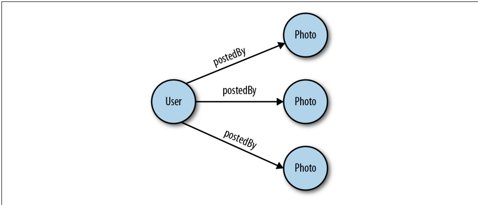
Figure 4-2. One-to-many connection
