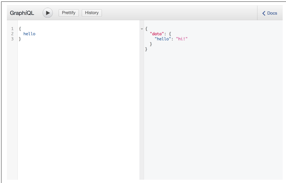
Figure 3-3. GraphiQL
