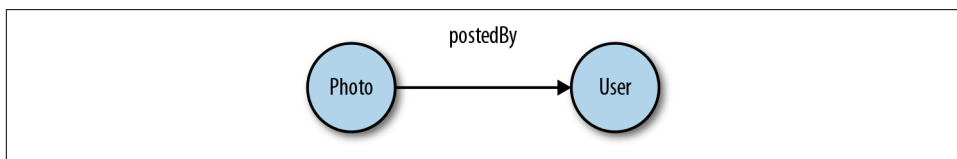
Figure 4-1. One-to-one connection
