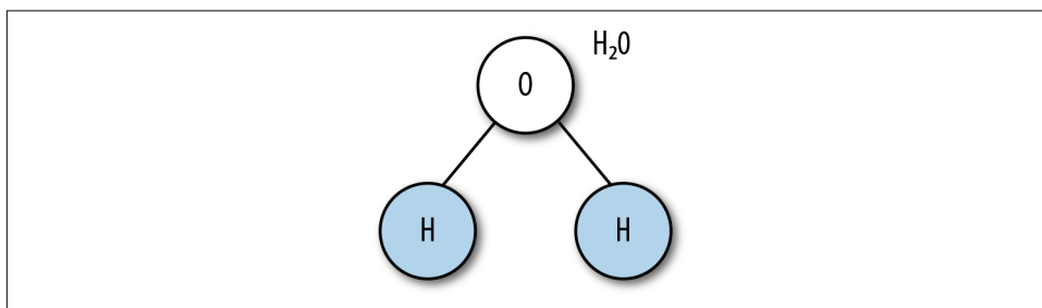
Figure 2-5. H 2 O diagram
