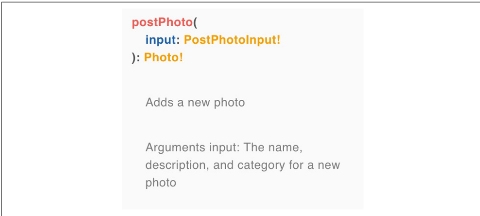
Figure 4-4. postPhoto Documentation
