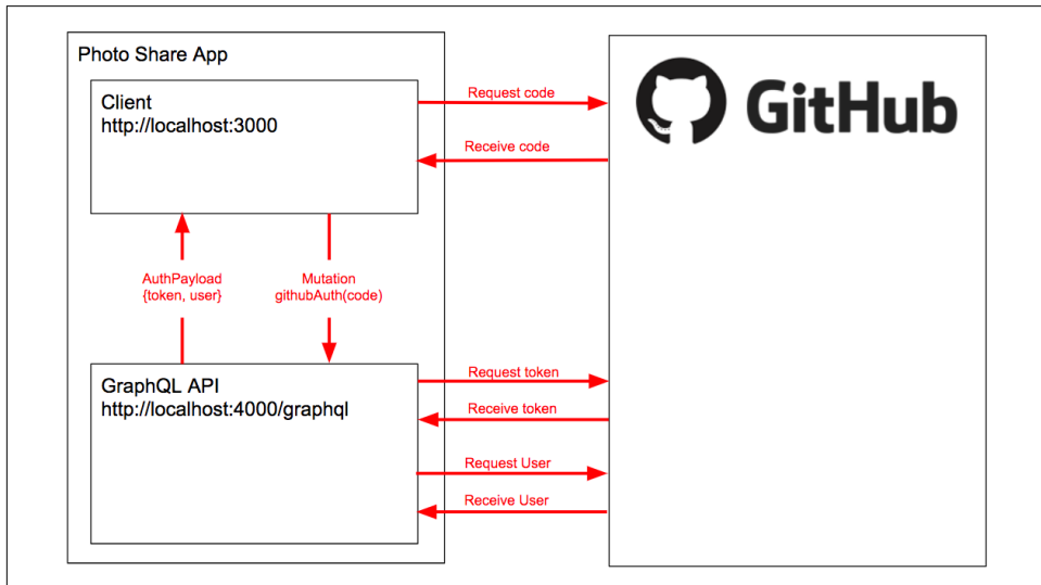
Figure 5-4. Authorization Process
