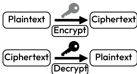
Figure 3.5 – Asymmetric encryption
