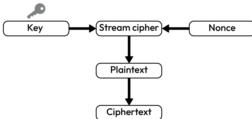
Figure 3.4 – Stream cipher
