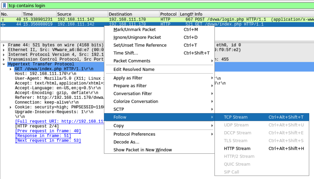
Figure 2.8 – Follow | TCP Stream within Wireshark
