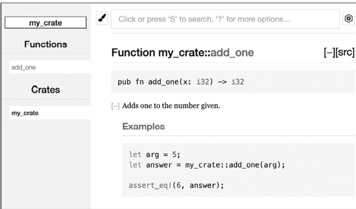
Figure 14-1: HTML documentation for the add_one function
