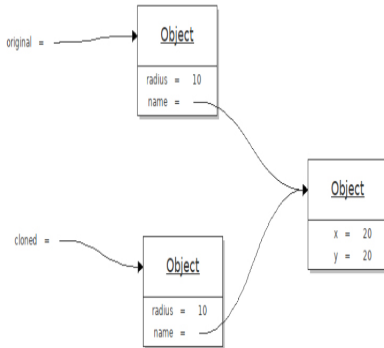
Figure 11-1 A shallow copy
