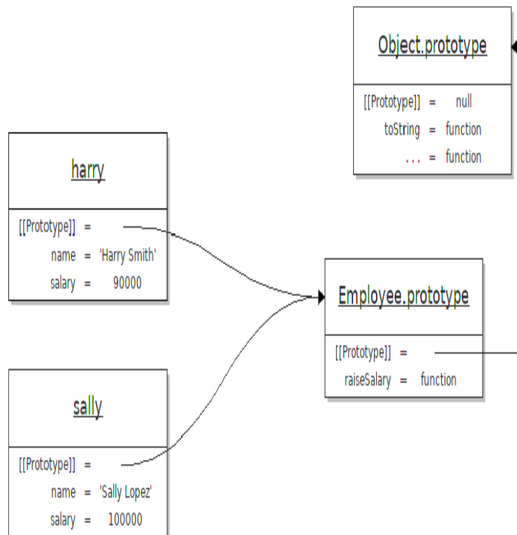
Figure 4-3 Objects created with a constructor
