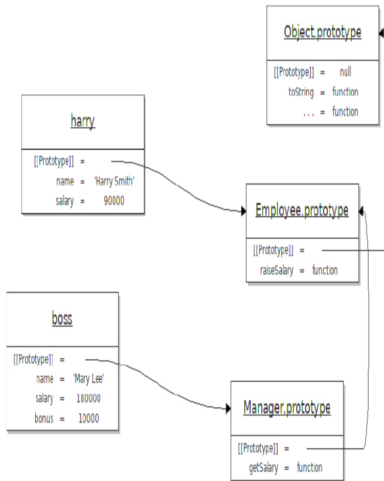
Figure 4-4 Prototype chain for inheritance
