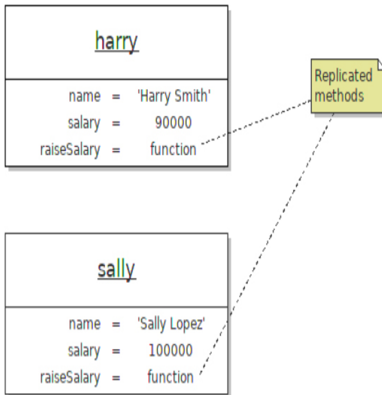
Figure 4-1 Objects with replicated methods
