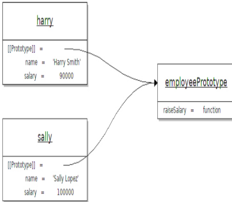
Figure 4-2 Objects with the same prototype
